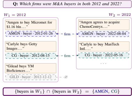
Figure 1: Query-operator QA: event tuples are latent in text (dashed), linked across articles only by shared typed attributes (color = firm; snippets illustrative).
