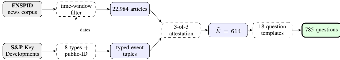
Figure 2: QO-BENCH construction pipeline. Date windows around S&P Capital IQ events filter the FNSPID (Dong et al., 2024) corpus; 3-of-3 judge attestation aligns the two into the operational event set \hat{E} (614 single-article-attestable events), over which 18 templates instantiate the 785-question benchmark with deterministic gold denotations.
